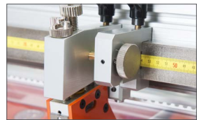
Fine positioning of the cutting blades (optional)
